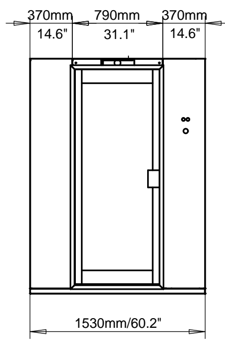
View B-B'
