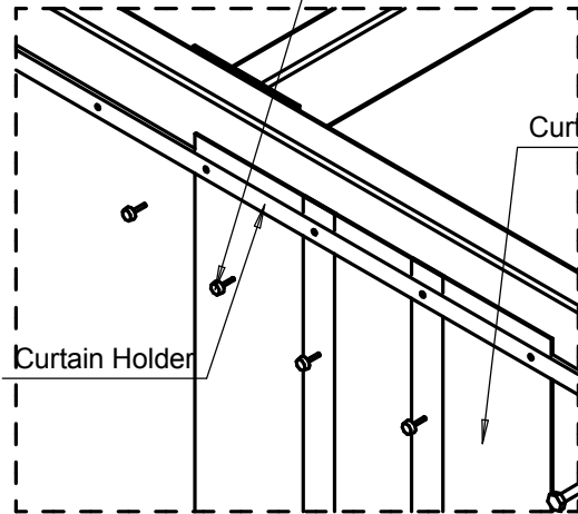
CURTAIN HOLDER CONNECTION DETAIL
