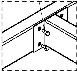
"T" CONNECTION DETAIL
