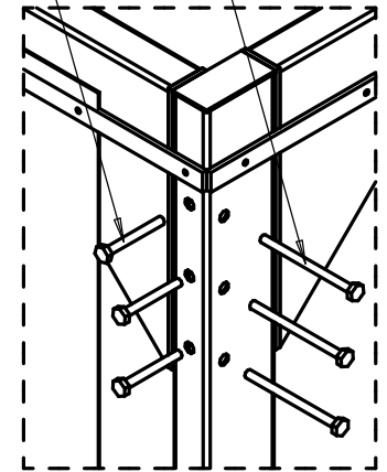
CORNER CONNECTION DETAIL
